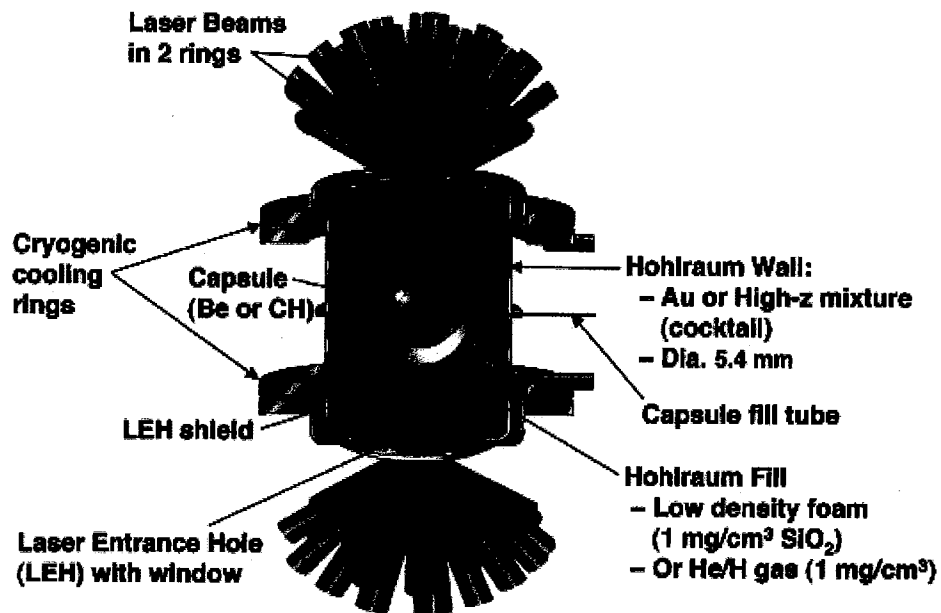
Fig. 23. 2005 Ignition Target Design for NIF.
