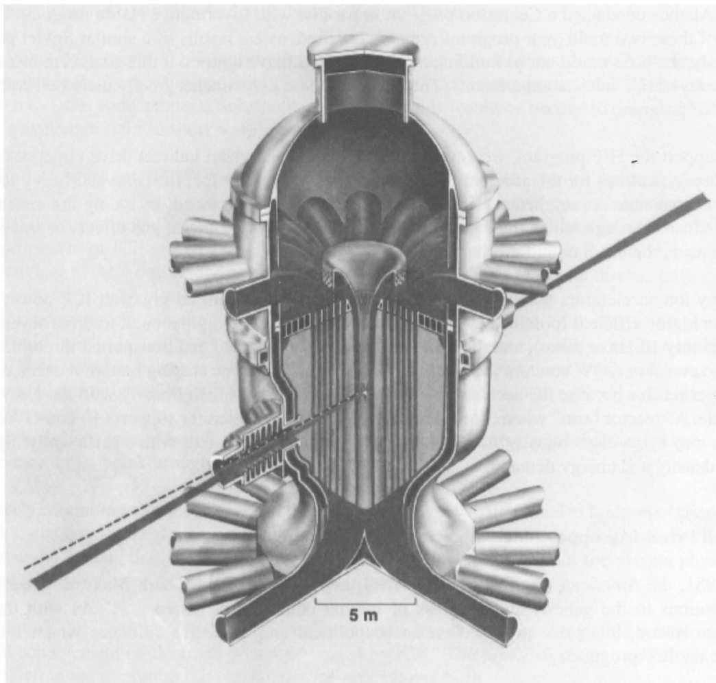
Fig. 17. ICF reactor with liquid lithium walls; five meter scale corresponds to a 1000 megawatt reactor.
