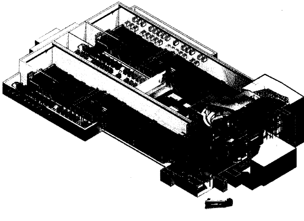
Fig. 21. Cutaway drawing of the NIF laser and target chamber area (Note truck which indicates scale of NIF).
