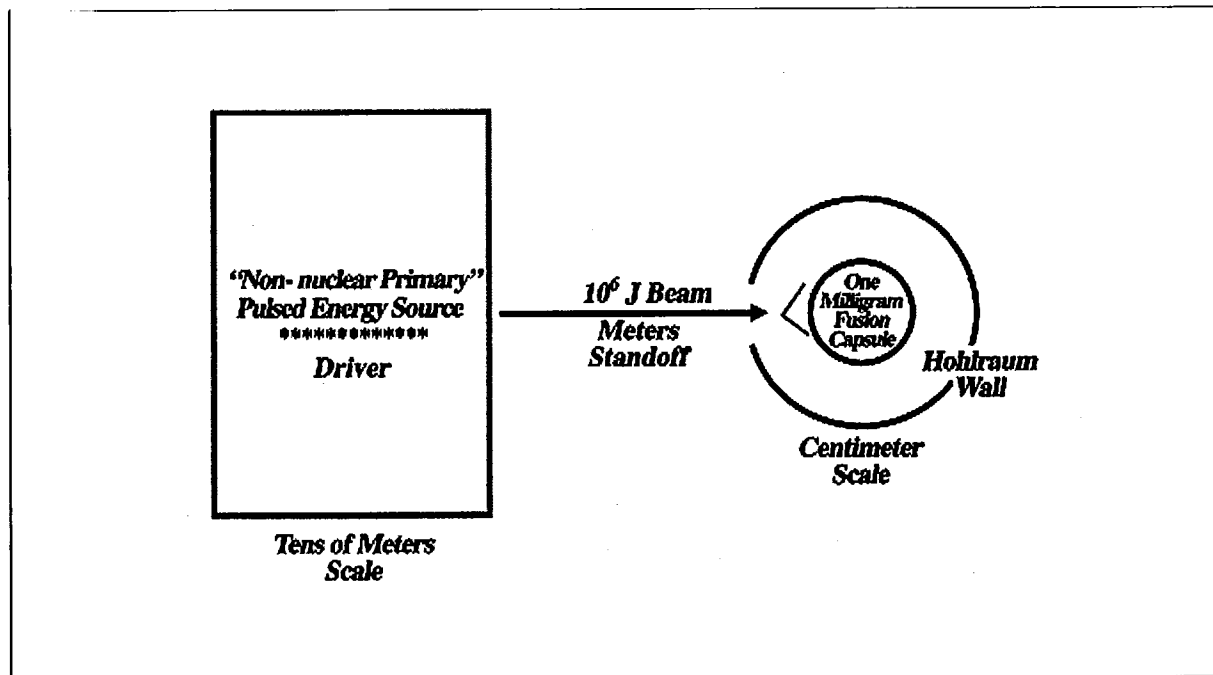
Fig. 4. Non-nuclear primary/indirect drive scheme (1960).
