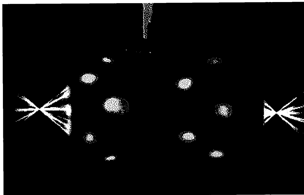
Fig. 19. Nova indirect-drive target experiment: ten hot spots are generated by focusing of ten Nova laser beams inside the tiny gold hohlraum (scale several mm).
