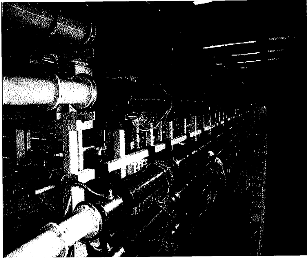
Fig. 13. Twenty beam, 10-kilojoule, 1micron wavelength Shiva laser.
