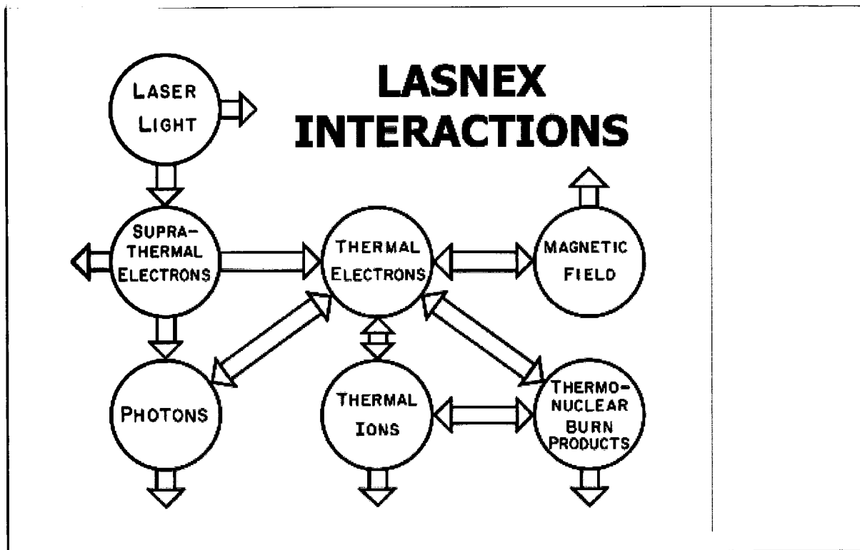
Fig. 9. LASNEX Target Design Code.
